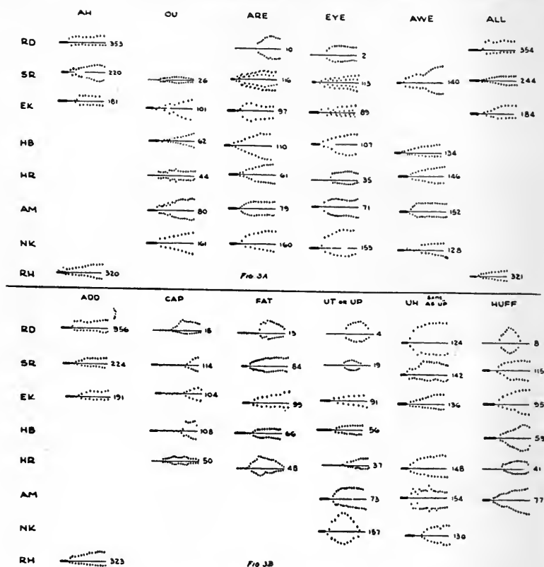
FIG. 3. Tracings of oscillograms of speech sounds.
